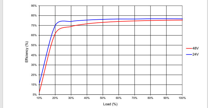
NCS12D4805C
