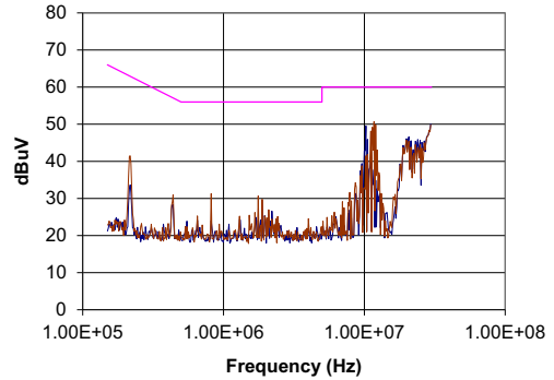
NCS12D4805C
