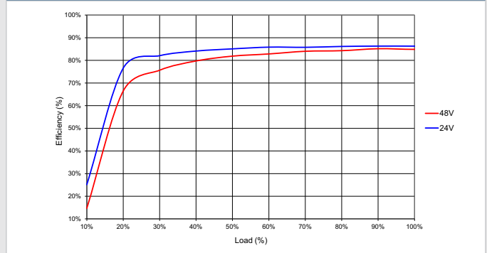
NCS12D4815C
