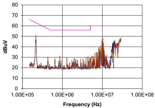
NCS12S4812C
