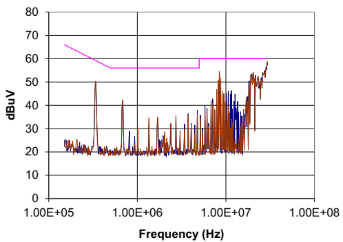
NCS12S4812C
