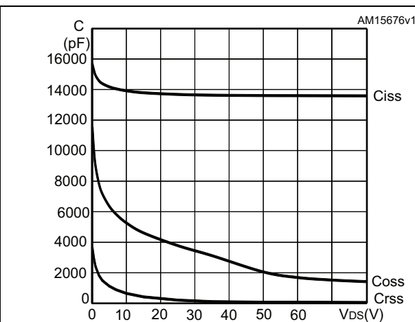
Figure 13. Capacitance variations
