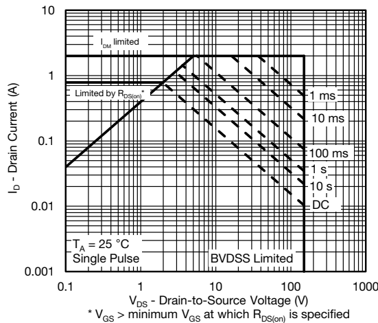
Safe Operating Area at T_A = 25\text{ °C}
