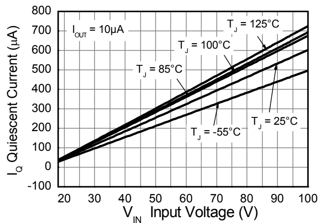
Quiescent Current
