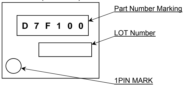
HTSOP-J8(TOP VIEW)
