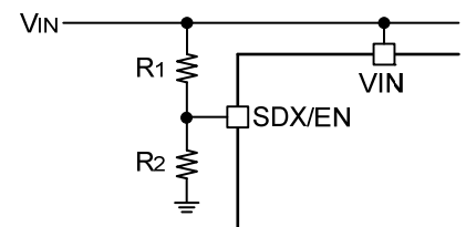
Figure .26 Enable Control with VIN terminal
