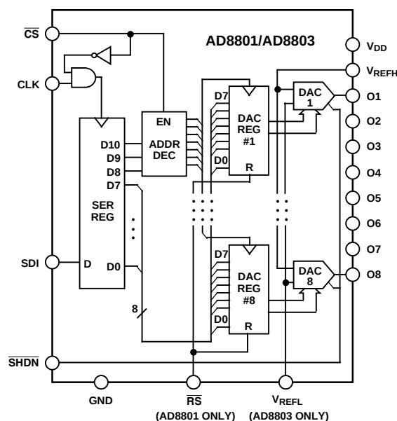
Figure 4. Block Diagram
