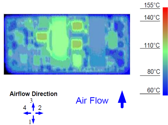
Figure 12. Thermal Image for Airflow Direction 3 (21A output, 55°C ambient, 200 LFM, typical Vin, open frame, socket interface)
