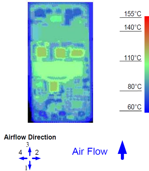
Figure 14. Thermal Image for Airflow Direction 2 (18.8A output, 55°C ambient, 200 LFM, typical Vin open frame, socket interface)
