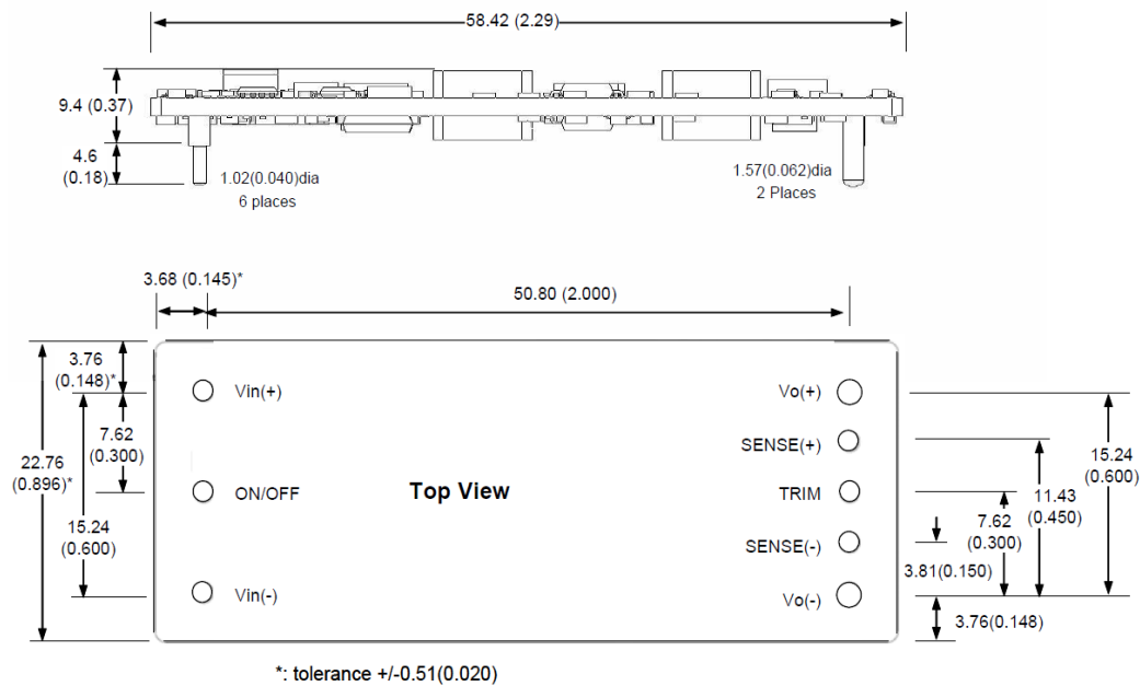
Figure 21. Converter with Open frame option
