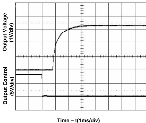
Figure 4. Start-Up from Enable Control (Typical Input voltage and zero load)
