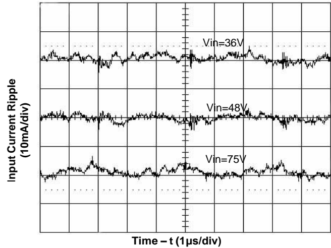
Figure 6. Input Reflected Ripple at Full Load
