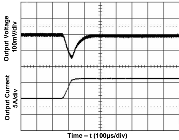
Figure 8. Transient Load Response
