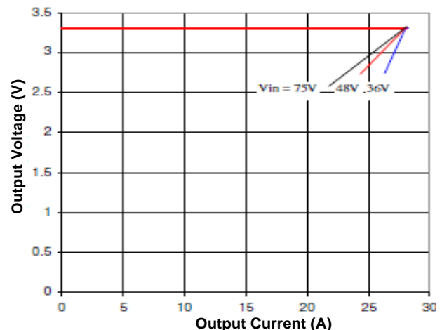
Figure 10. Output Characteristics
