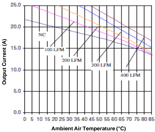
Figure 13. Current Derating Curve for Airflow Direction 2 (Ref. Figure 14 for Airflow Direction; Vin = 48V, open frame unit)
