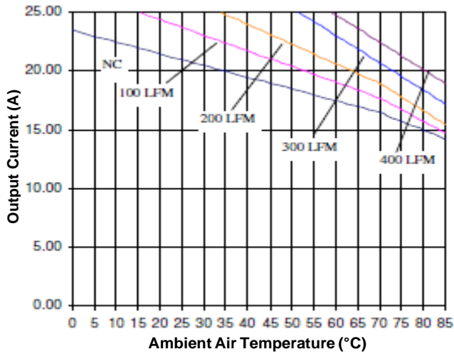
Figure 11. Current Derating Curve for Airflow Direction 3 (Ref. Figure 12 for Airflow Direction; Vin = 48V, open frame unit)
