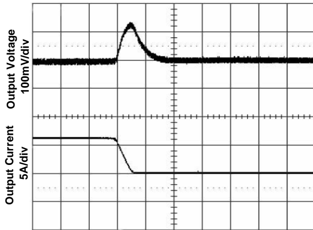
Figure 7. Transient Load Response
