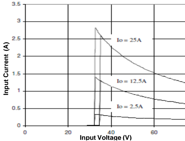
Figure 9. Input Characteristics
