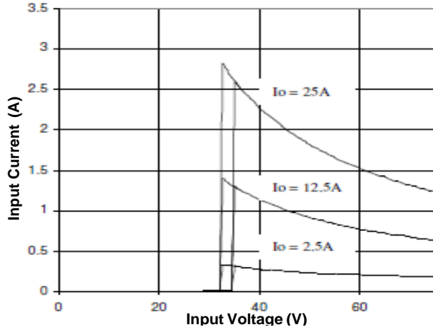
Figure 9. Input Characteristics
