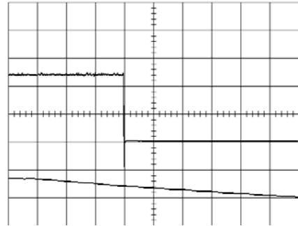
Shut-down enabled by disconnecting V_i at: T_{ref} = +25^\circ\text{C} , I_O = 18\text{ A} resistive load, V_i = 12.0\text{ V} . Top trace: output voltage (1.0 V/div.). Bottom trace: input voltage (2 V/div.). Time scale: 5.0 ms/div.
