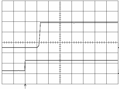
Start-up enabled by connecting V_i at: T_{ref} = +25^\circ\text{C} , I_O = 18\text{ A} resistive load, V_i = 12.0\text{ V} . Top trace: output voltage (0.5 V/div.). Bottom trace: input voltage (10 V/div.). Time scale: 10 ms/div.
