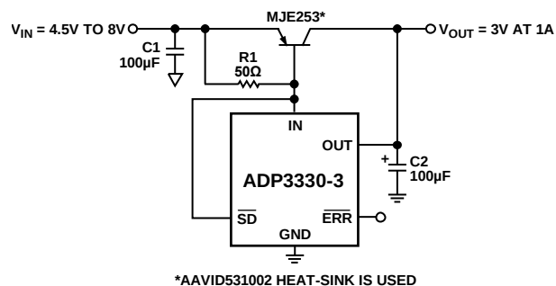
Figure 28. High Output Current Linear Regulator
