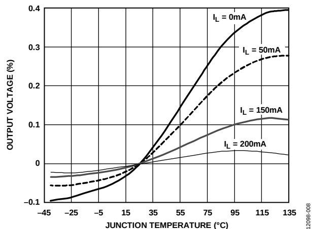
Figure 8. Output Voltage Variation Percent vs. Junction Temperature
