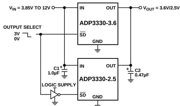
Figure 27. Crossover Switch
