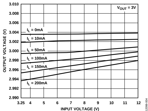
Figure 4. Line Regulation Output Voltage vs. Input Voltage
