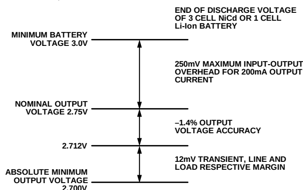
Figure 26. LDO Budgeting for a 3 Cell NiCd/1 Cell Li-Ion Supply
