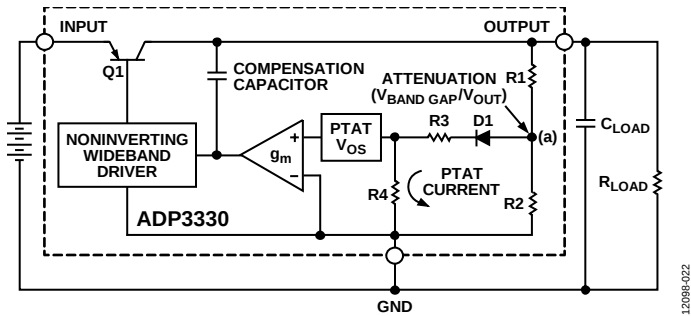
Figure 22. Functional Block Diagram
