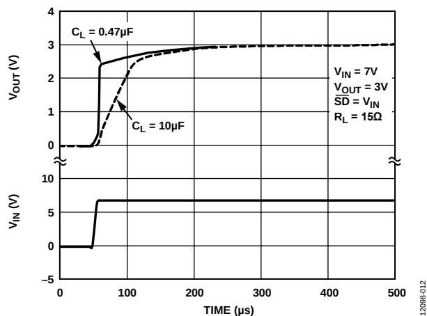
Figure 12. Power-Up Response
