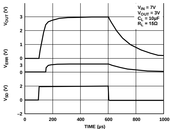
Figure 18. Turn On/Turn Off Response
