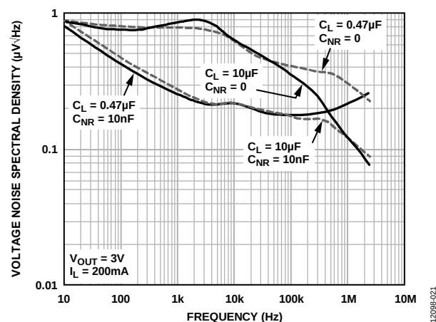
Figure 21. Output Noise Density
