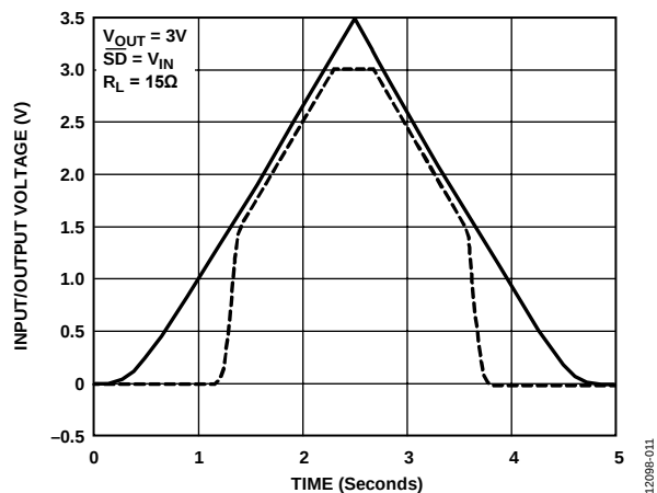
Figure 11. Power-Up/Power-Down
