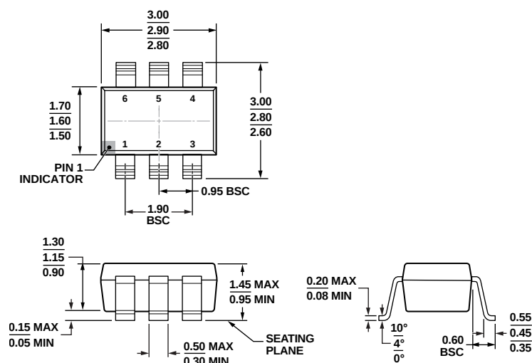
Figure 29. 6-Lead Small Outline Transistor Package [SOT-23] RJ-6
