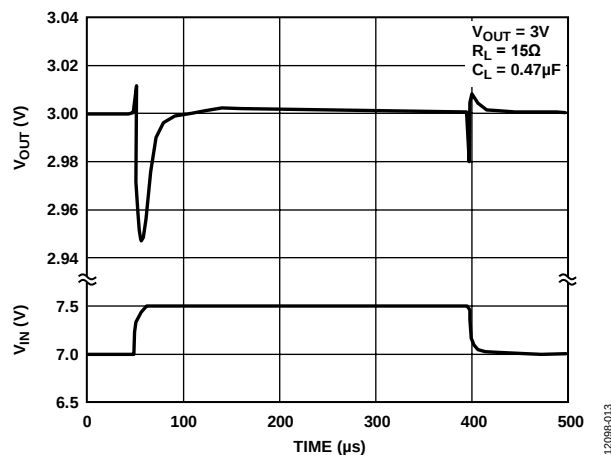
Figure 13. Line Transient Response, C_L = 0.47 \mu F
