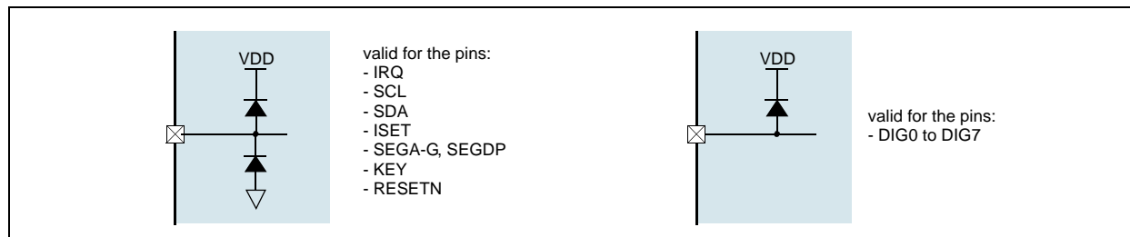
Figure 17. ESD Structure
