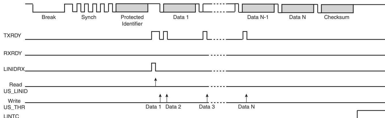
Figure 40-48. Slave Node Configuration, NACT = PUBLISH
