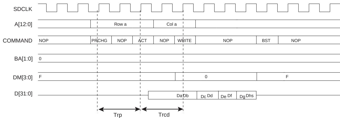
Figure 31-7. Burst Write Access, Row Closed, SDR-SDRAM Device
