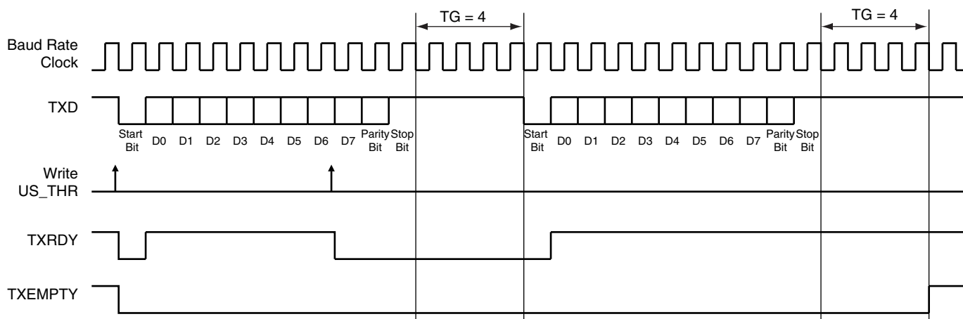
Figure 40-23. Timeguard Operations
