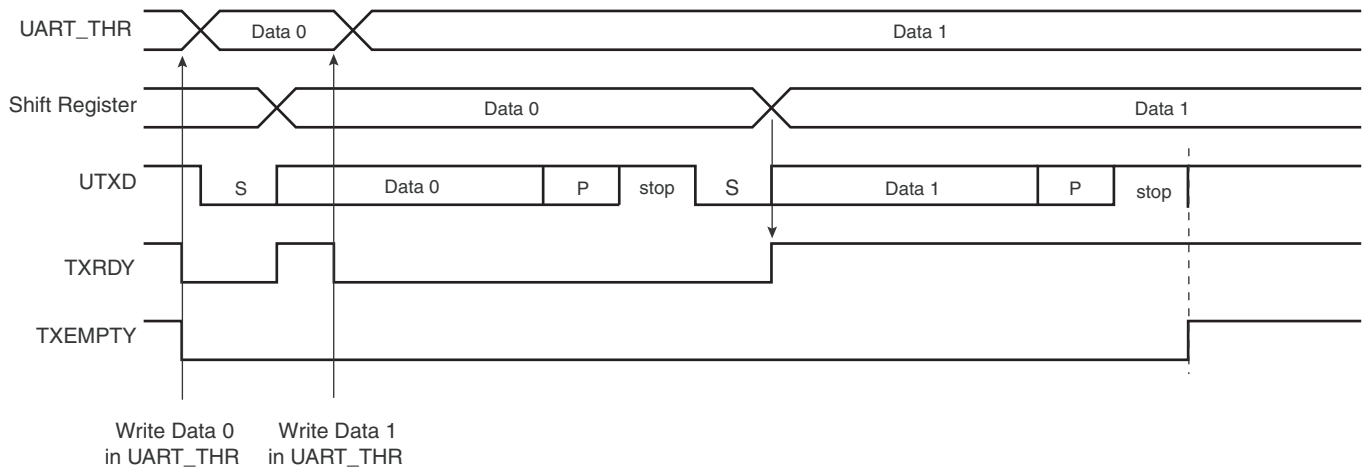
Figure 41-10. Transmitter Control
