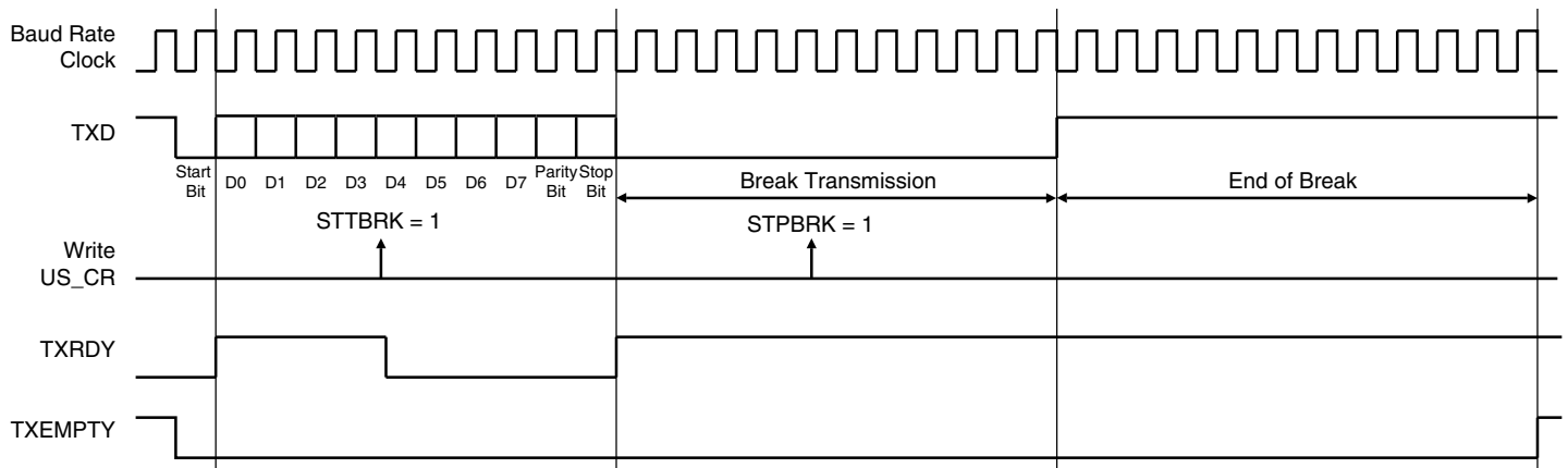
Figure 40-26. Break Transmission
