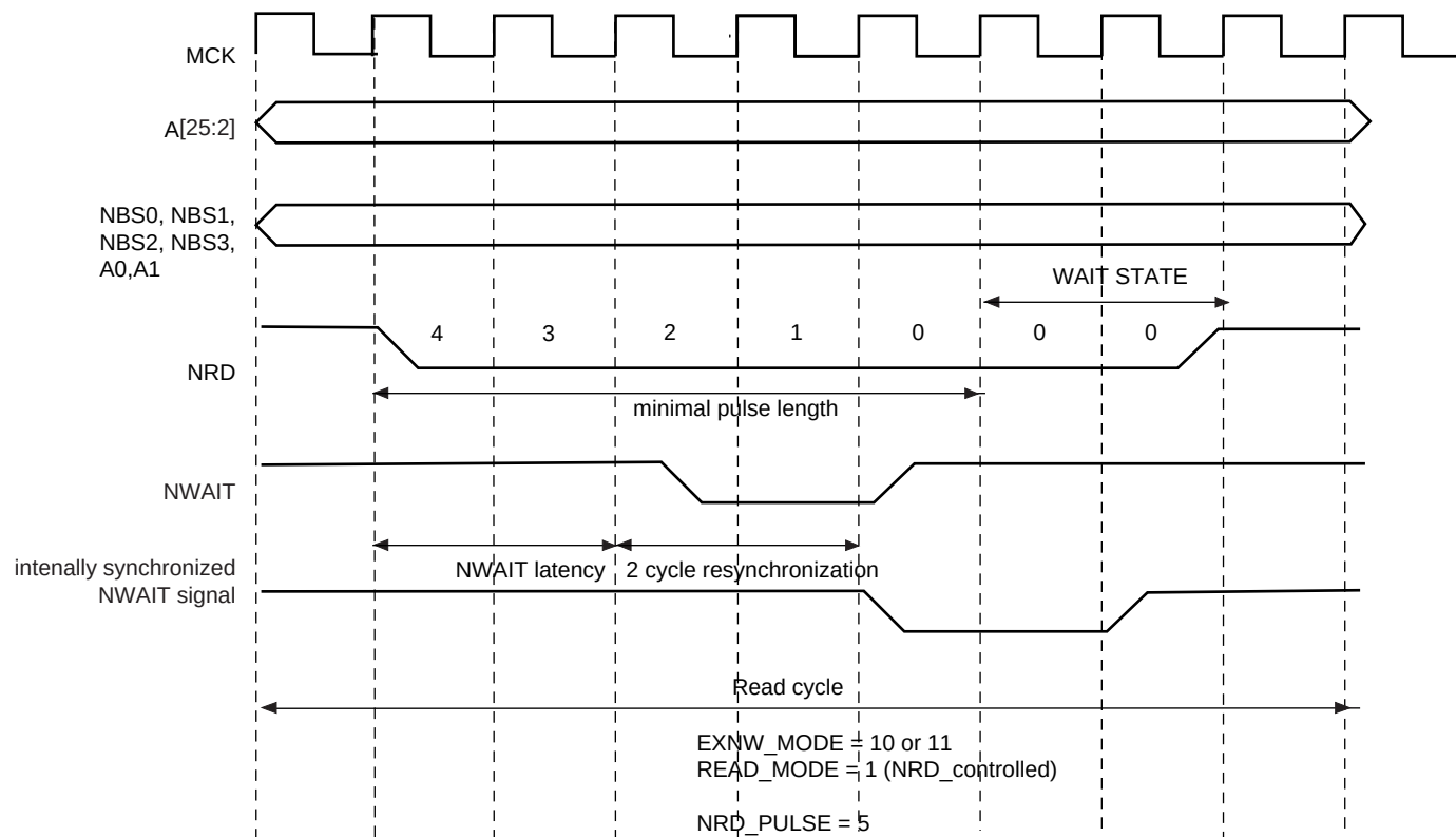
Figure 30-30. NWAIT Latency
