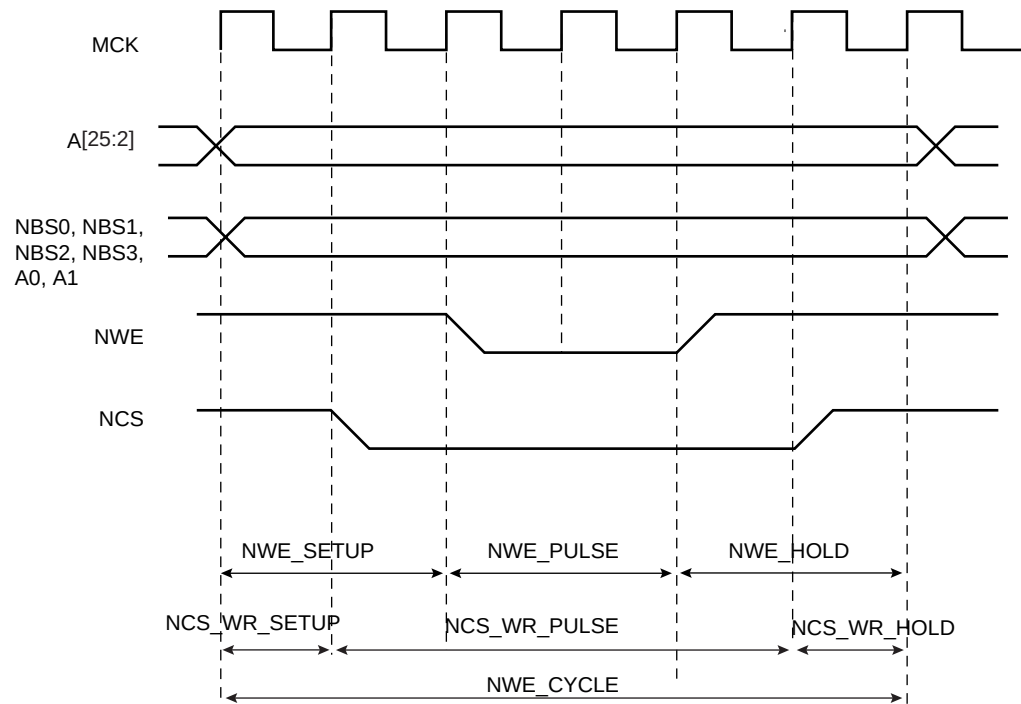
Figure 30-12. Write Cycle
