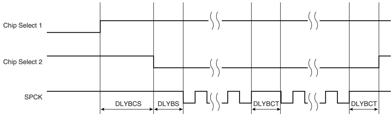
Figure 36-8. Programmable Delays
