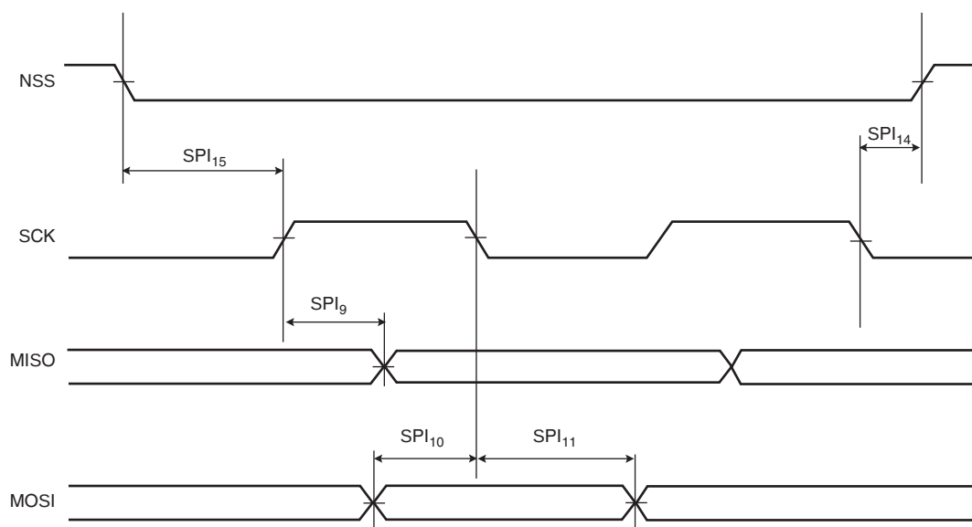
Figure 48-21. USART SPI Slave mode: (Mode 0 or 3)
