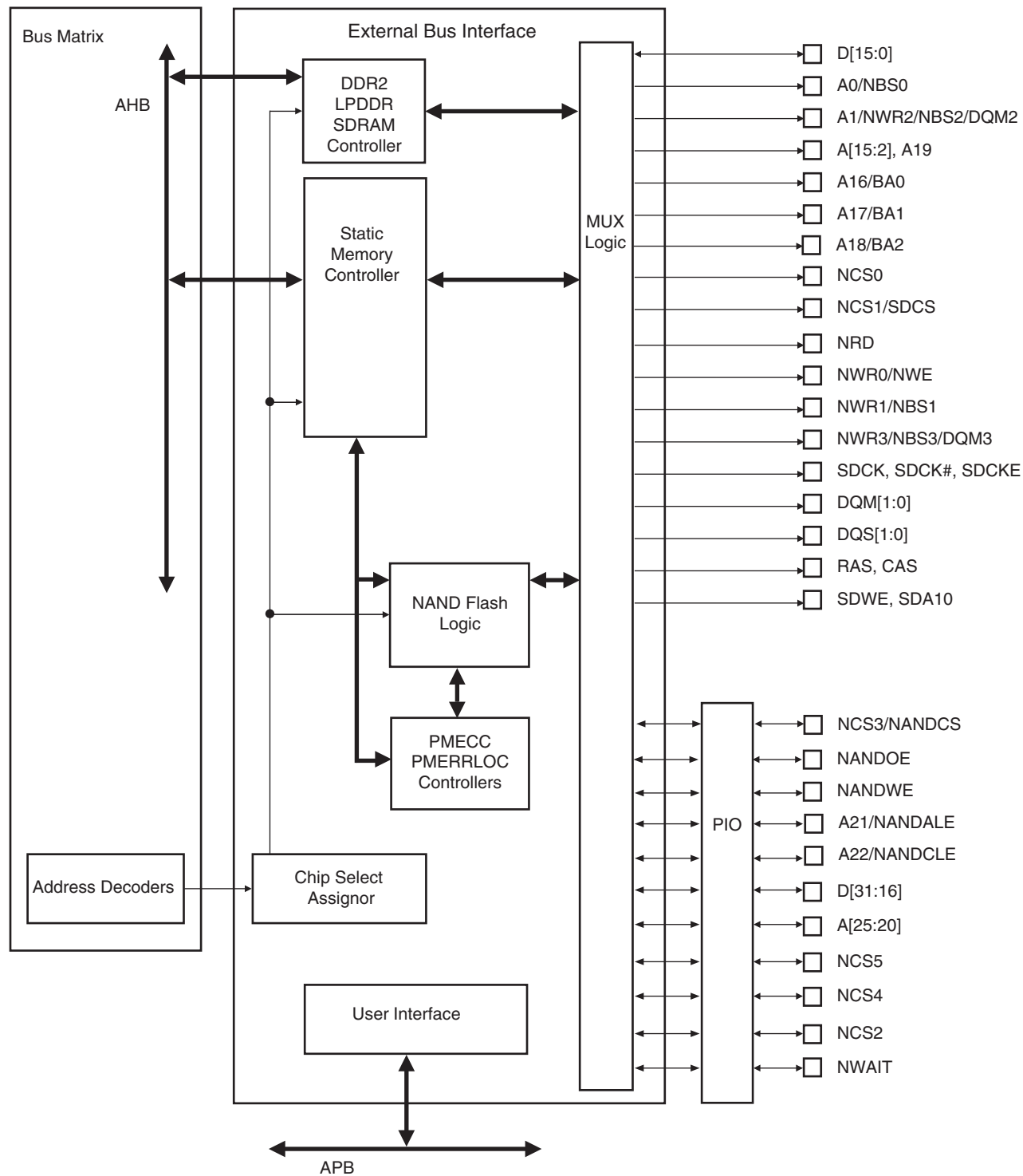
Figure 27-1. Organization of the External Bus Interface
