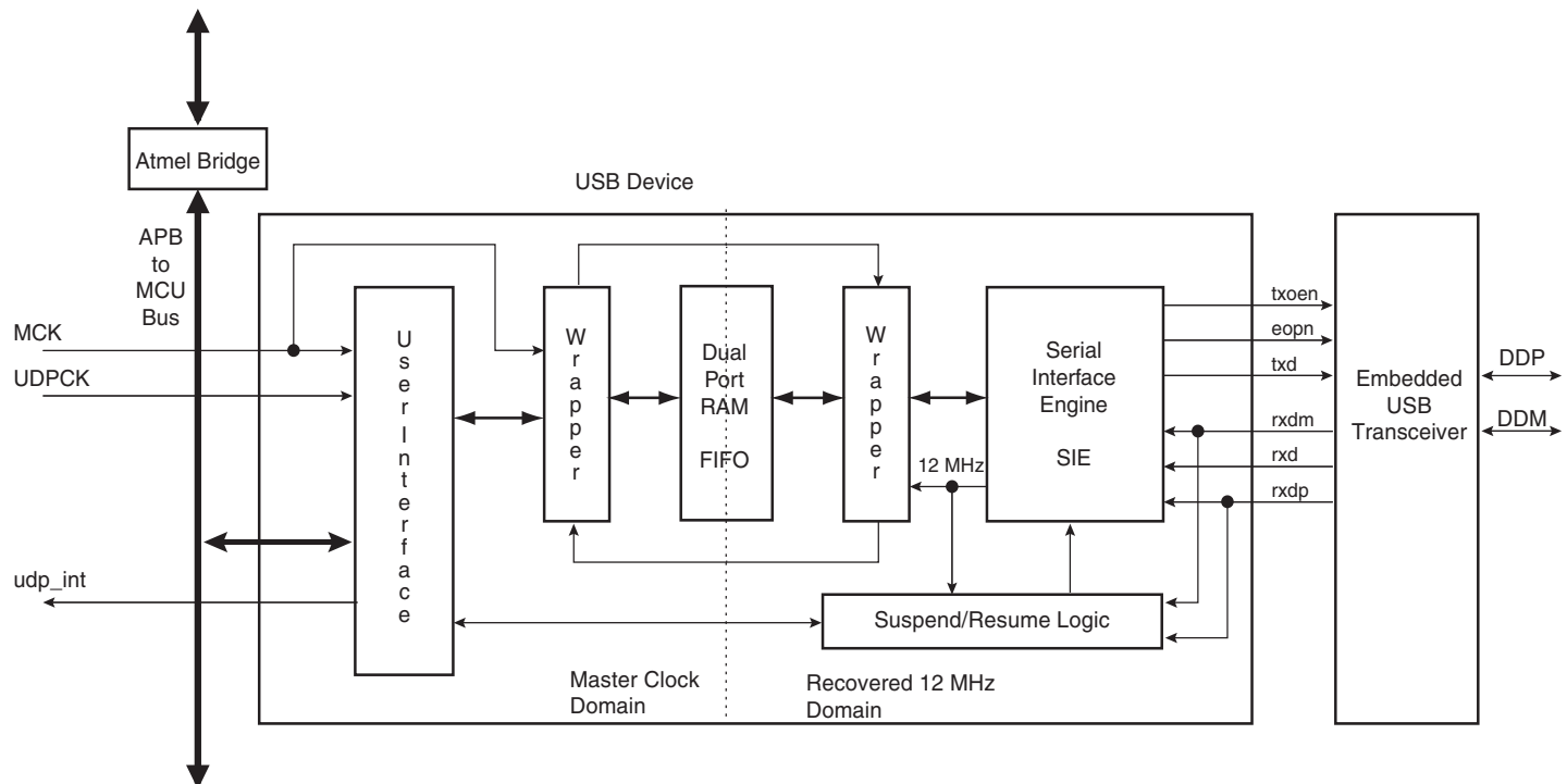
Figure 33-1. Block Diagram
