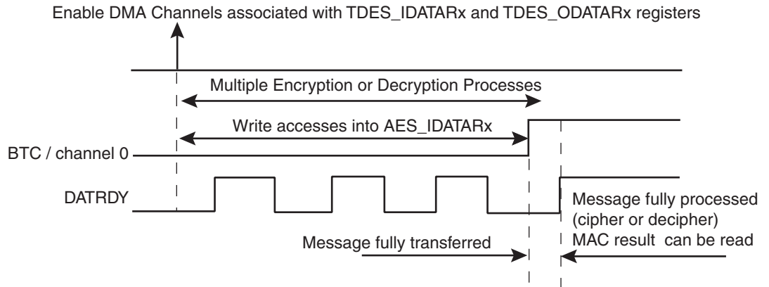
Figure 45-4. DMA transfer with LOD = 1
