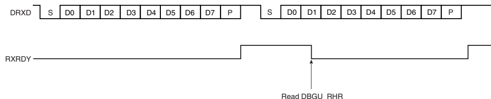
Figure 24-6. Receiver Ready
