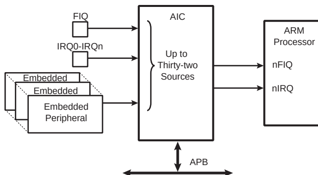
Figure 11-1. Block Diagram
