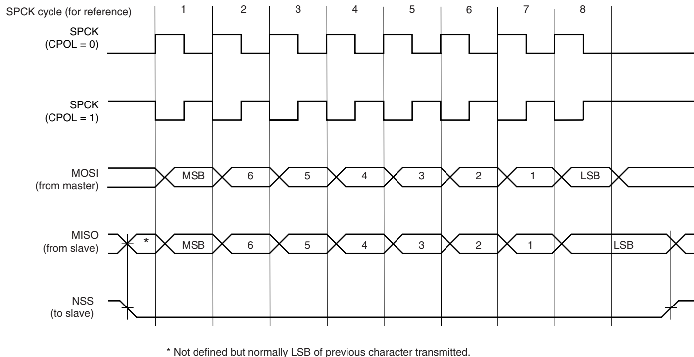
Figure 36-4. SPI Transfer Format (NCPHA = 0, 8 bits per transfer)
