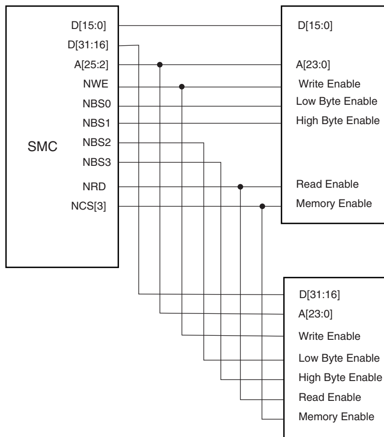
Figure 30-7. Connection of 2x16-bit Data Bus on a 32-bit Data Bus (Byte Select Option)
