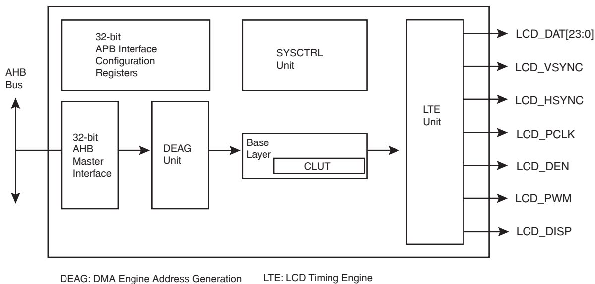
Figure 44-1. Block Diagram
