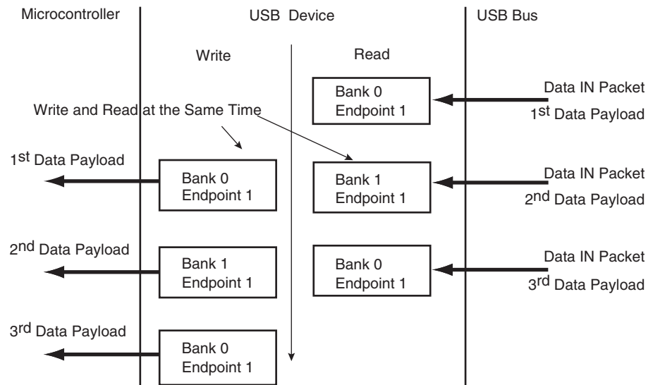
Figure 33-10. Bank Swapping in Data OUT Transfers for Ping-pong Endpoints
