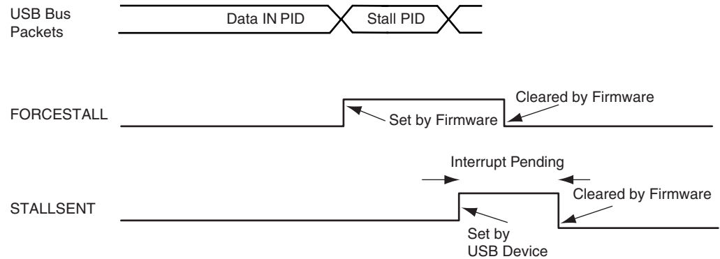
Figure 33-12. Stall Handshake (Data IN Transfer)
