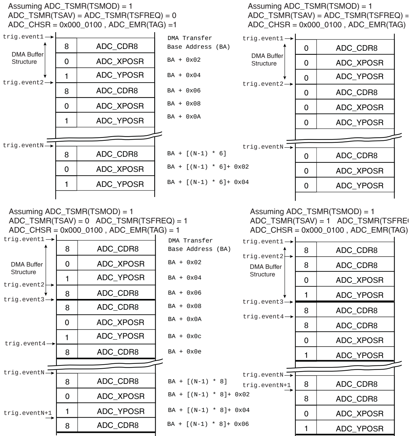
Figure 42-14. Buffer Structure when classic ADC and touchscreen channels are interleaved
