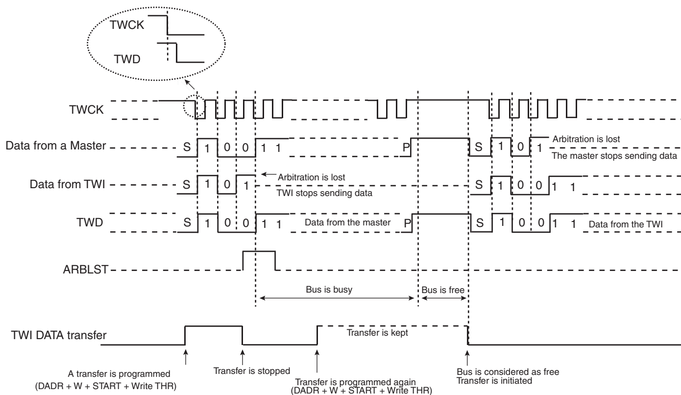
Figure 39-22. Arbitration Cases
