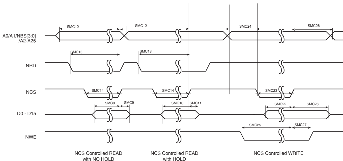
Figure 48-2. SMC Timings - NCS Controlled Read and Write
