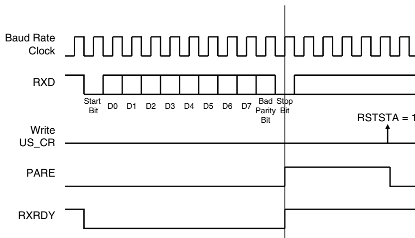
Figure 40-22. Parity Error
