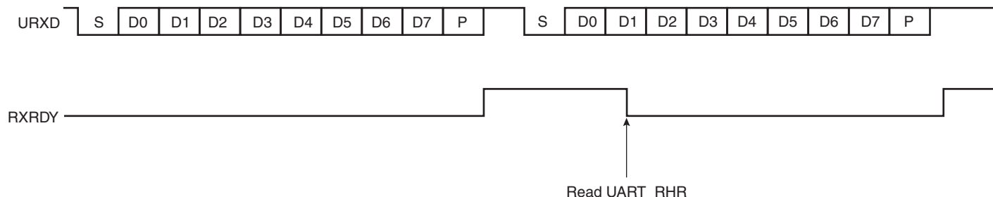
Figure 41-5. Receiver Ready
