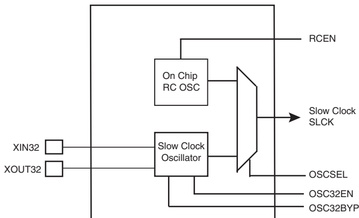
Figure 20-1. Block Diagram
