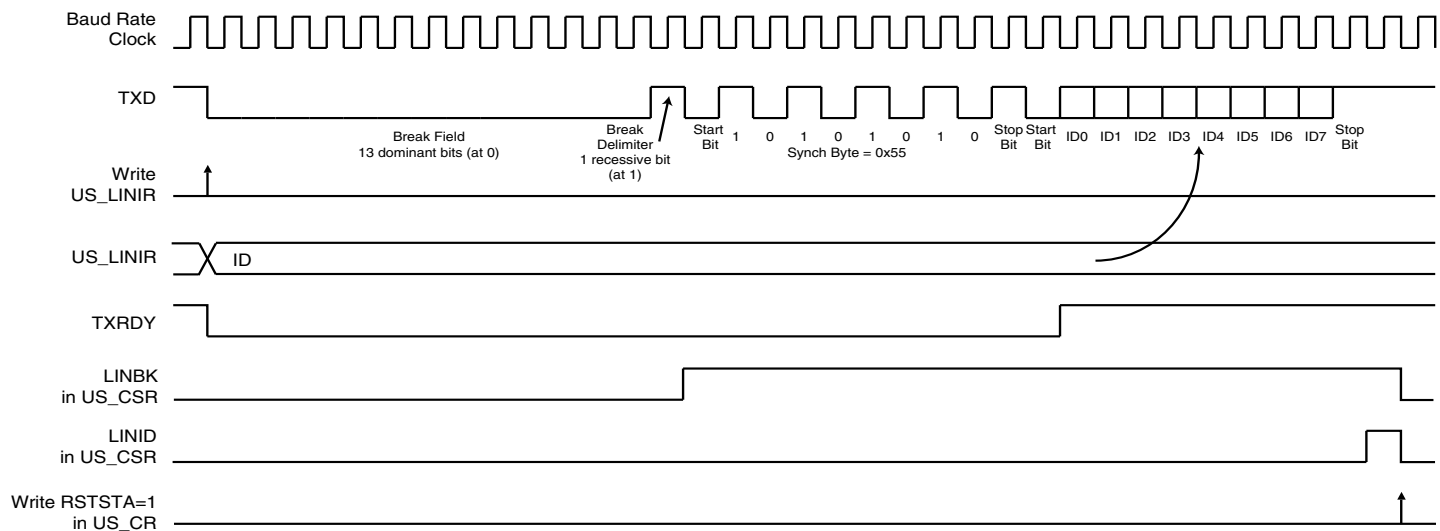
Figure 40-39. Header Transmission
