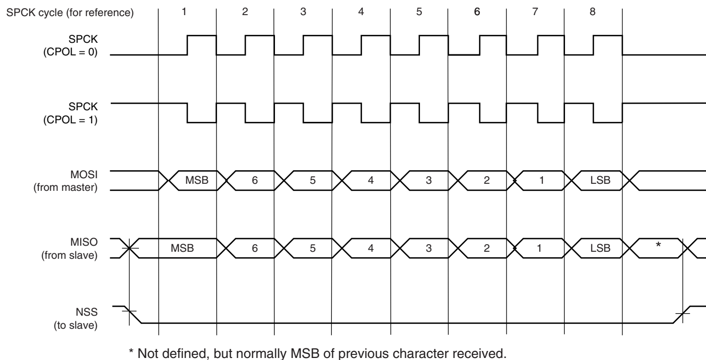
Figure 36-3. SPI Transfer Format (NCPHA = 1, 8 bits per transfer)
