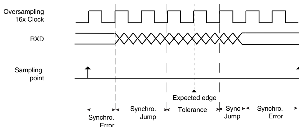
Figure 40-11. Bit Resynchronization
