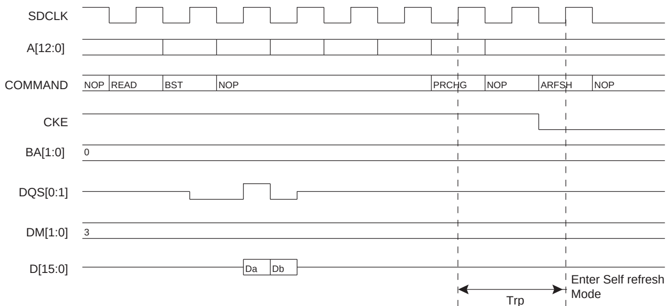
Figure 31-17. Self Refresh Mode Entry, Timeout = 0
