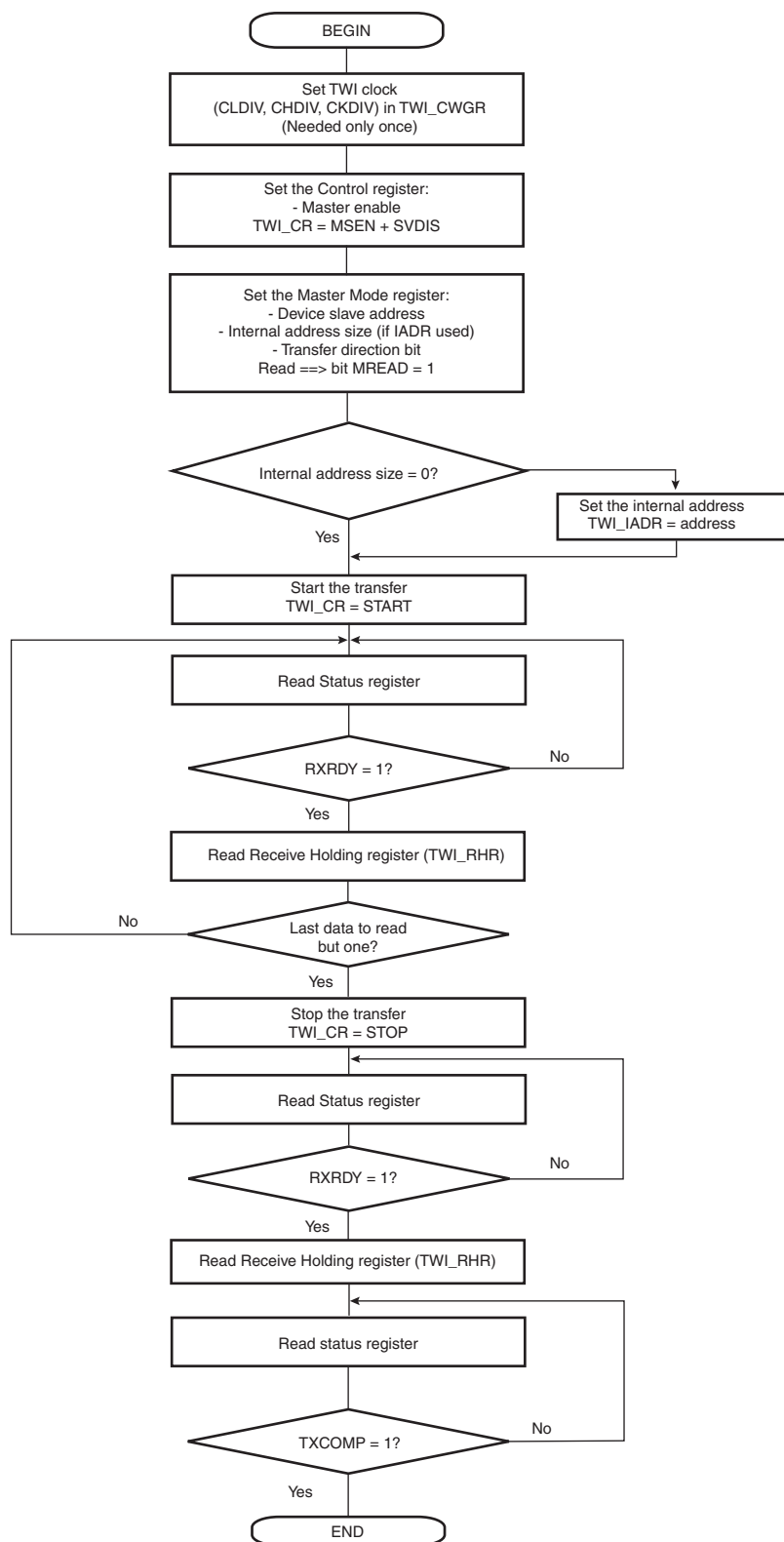
Figure 39-20. TWI Read Operation with Multiple Data Bytes with or without Internal Address
