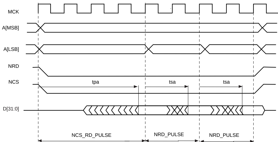
Figure 30-34. Page Mode Read Protocol (Address MSB and LSB are defined in Table 30-6)
