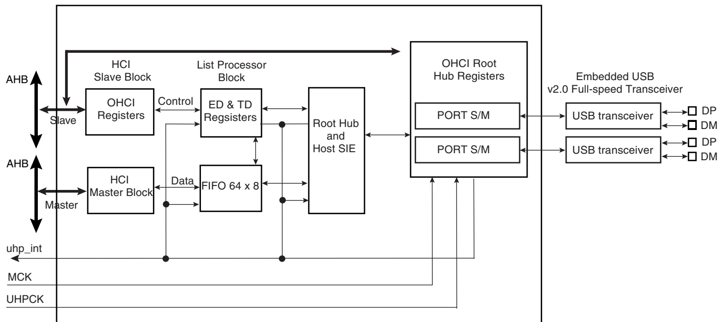
Figure 34-1. Block Diagram
