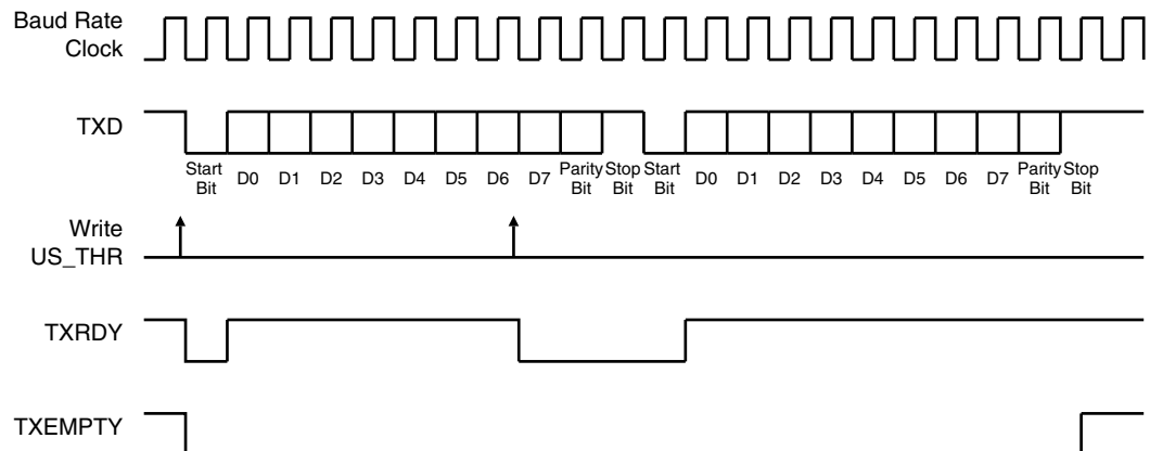
Figure 40-7. Transmitter Status
