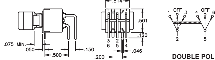
DOUBLE POLE
