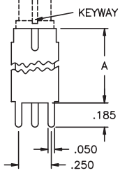
FRONT VIEW DOUBLE POLE
