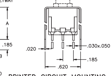
PRINTED CIRCUIT MOUNTING
