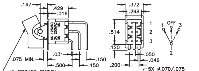
SINGLE POLE WITH J1 ROCKER
