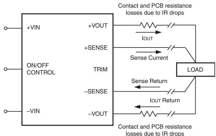
Figure 4. Remote Sense Circuit Configuration Sense is included only on models IRS-3.3/15-Q48 and IRS-5/10-Q48.
