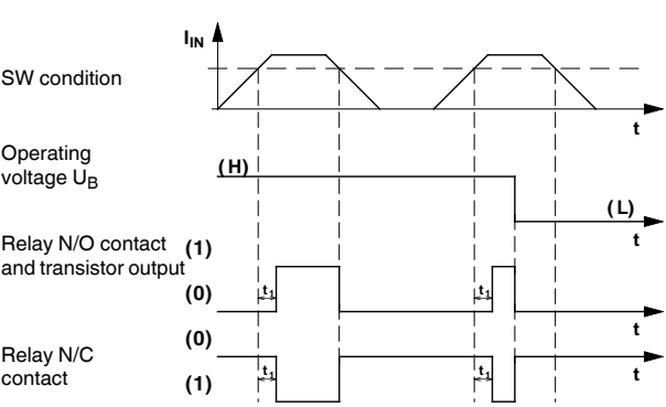
Figure 5 Function diagram: Operating current-controlled when above threshold value
