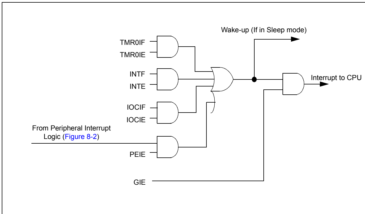
FIGURE 8-1: INTERRUPT LOGIC
