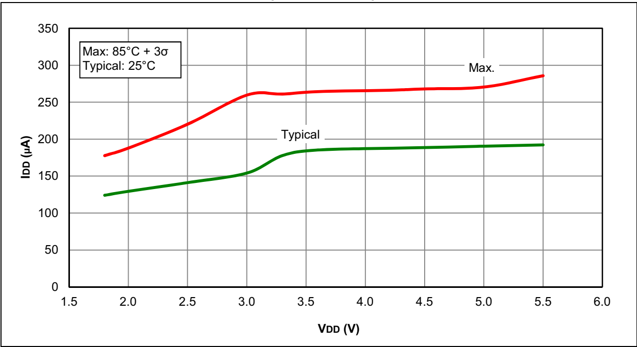
FIGURE 31-22: I_{DD} , MFINTOSC MODE ( F_{osc} = 500\text{ kHz} ), PIC12F1822 AND PIC16F1823 ONLY
