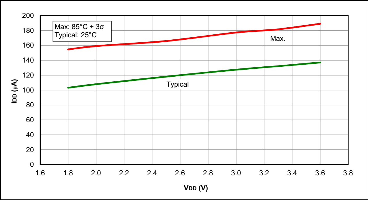
FIGURE 31-21: I_{DD} , MFINTOSC MODE ( F_{osc} = 500\text{ kHz} ), PIC12LF1822 AND PIC16LF1823 ONLY
