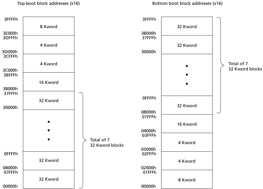
Figure 7: Block Addresses – x16
