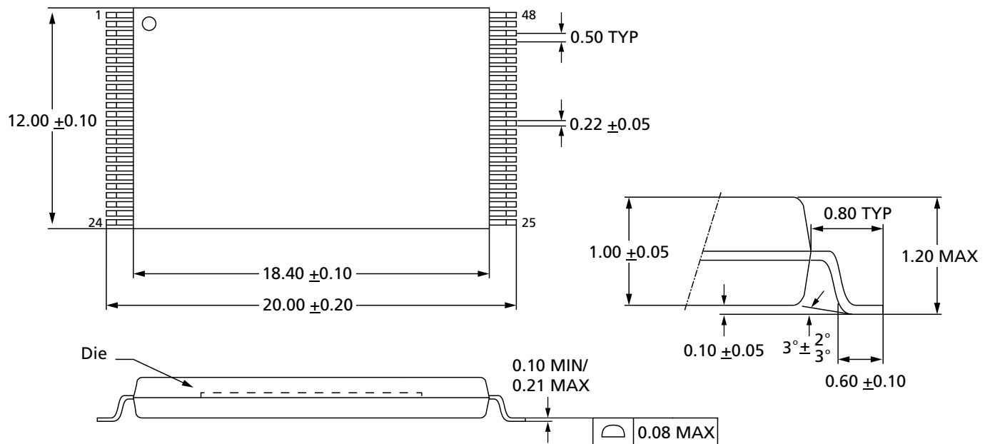
Figure 25: 48-Lead TSOP – 12mm x 20mm
