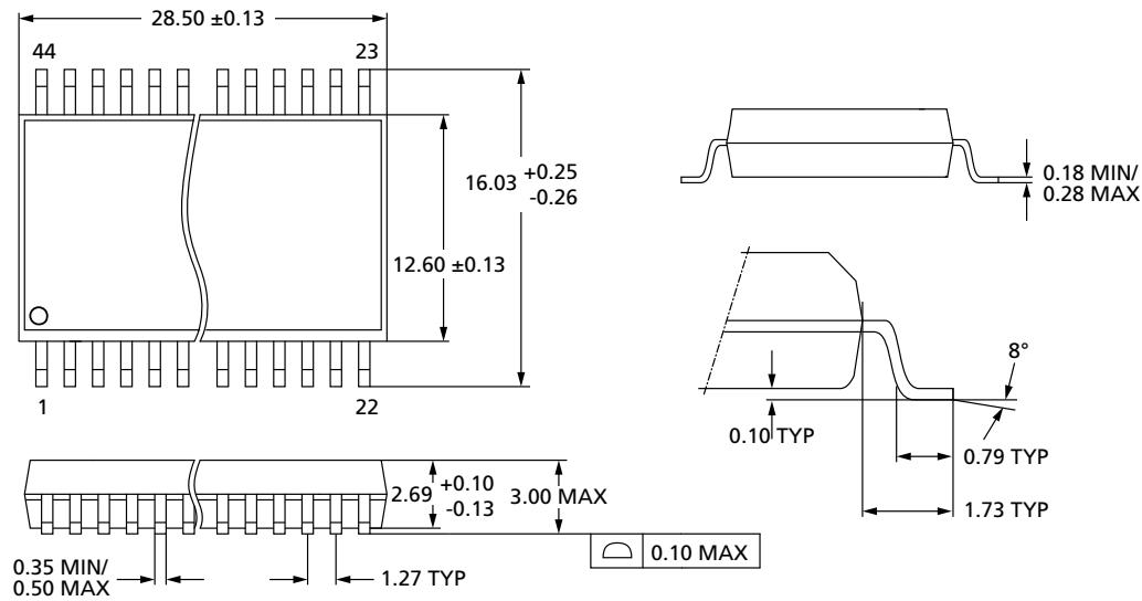
Figure 26: 44-Lead Small-Outline – 500 Mil
