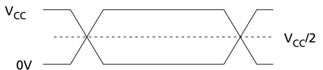
Figure 19: AC Measurement I/O Waveform
