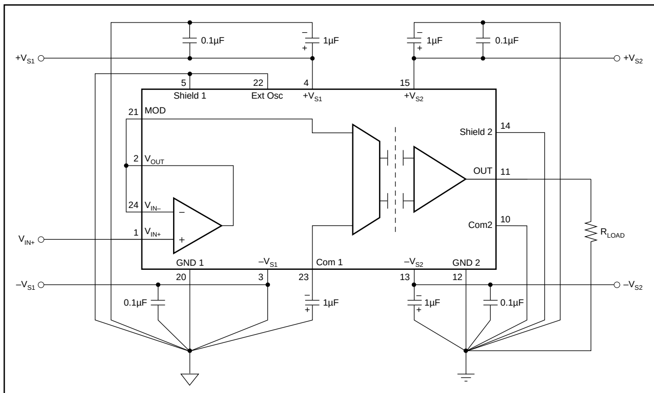
FIGURE 1. Basic Connections.
