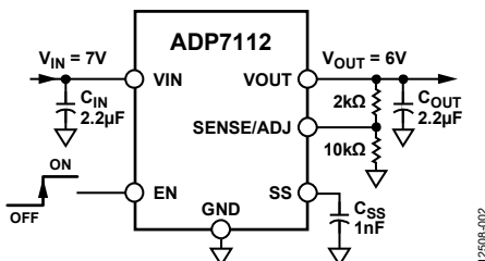
Figure 2. ADP7112 with 5 V Output Adjusted to 6 V
