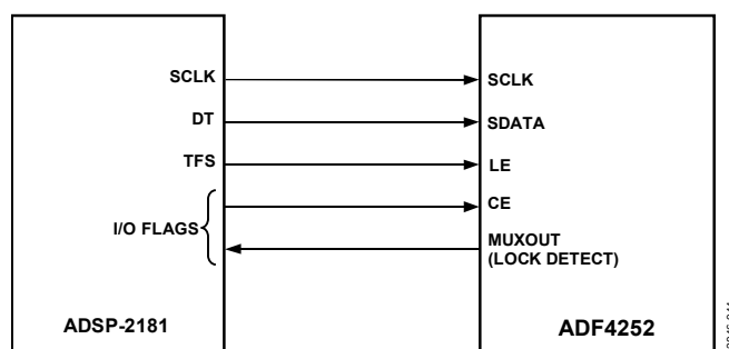
Figure 43. ADSP-2181 to ADF4252 Interface
