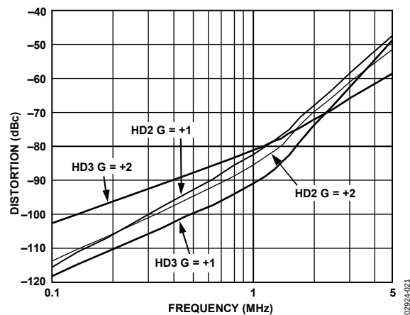
Figure 21. Harmonic Distortion vs. Frequency for Various Gains
