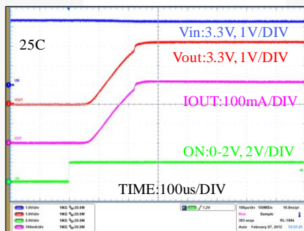
Figure 20. Turn-On Response (V IN =3.3 V, C OUT =0.1 μF, R L =10 Ω)
