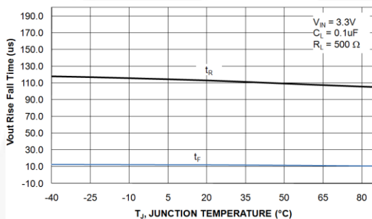
Figure 18. V OUT Rise/Fall Time vs. Temperature (R L =500 Ω)
