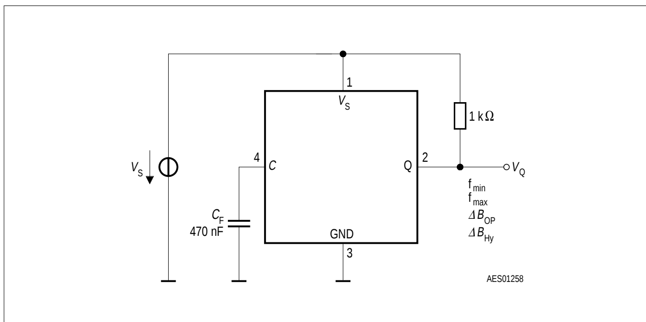
Figure 4 Test Circuit 2
