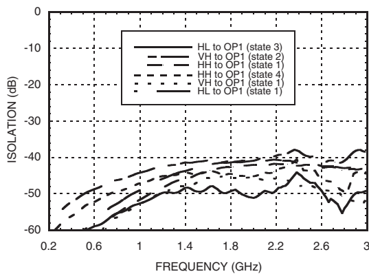
Isolation When VL is Connected to OP1*
