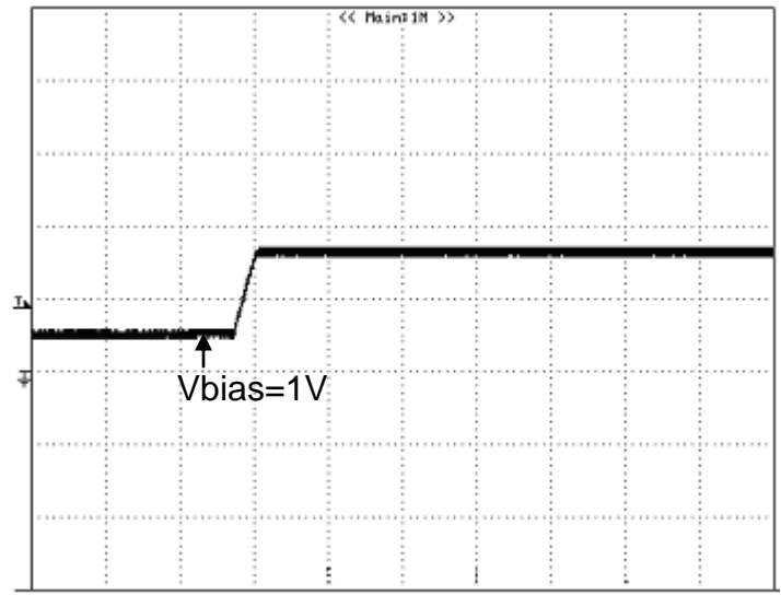
Figure 22: Turn on with Prebias 5V_{in} , 3.3V/0A out, V_{bias} = 1.0V_{dc} 2V/div , 10mS/div
