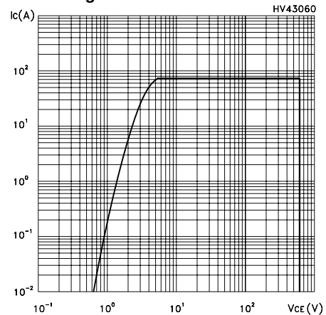
Figure 13: Turn-off SOA
