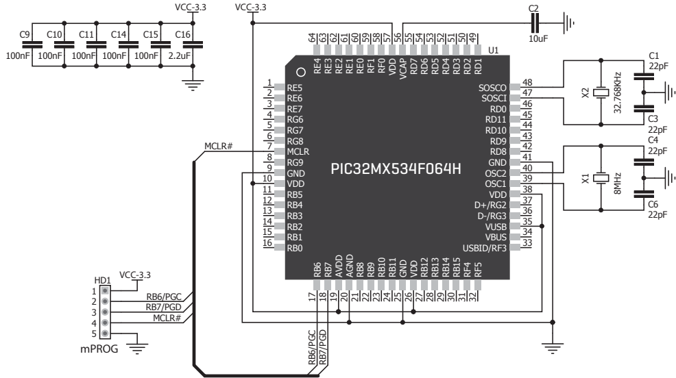
Figure 4-10: mikroProg™ connection schematic
