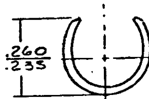
SECT. B-B
