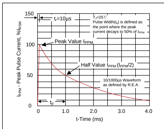
Figure 2. 10/1000 \mu s Pulse Waveforms
