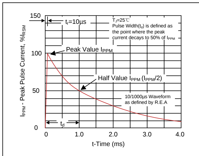
Figure 2. 10/1000μs Pulse Waveforms
