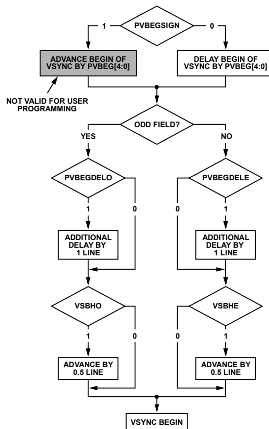
Figure 43. PAL VSYNC Begin
