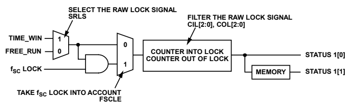
Figure 19. Lock Related Signal Path
