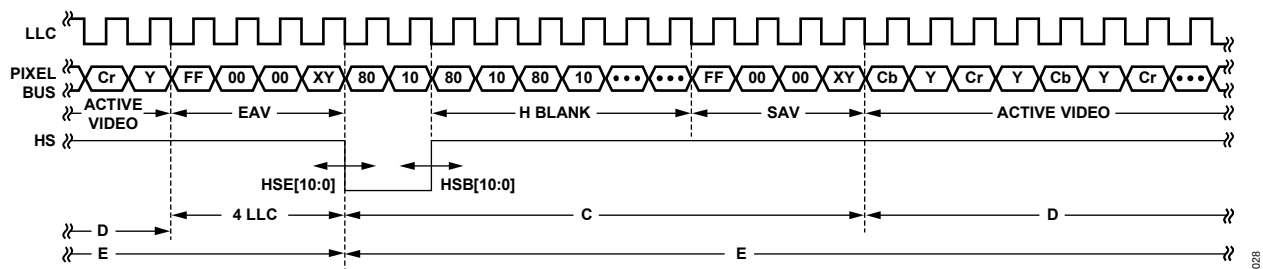
Figure 35. HS Timing
