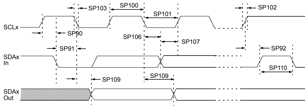
FIGURE 30-21: I 2 C BUS DATA TIMING
