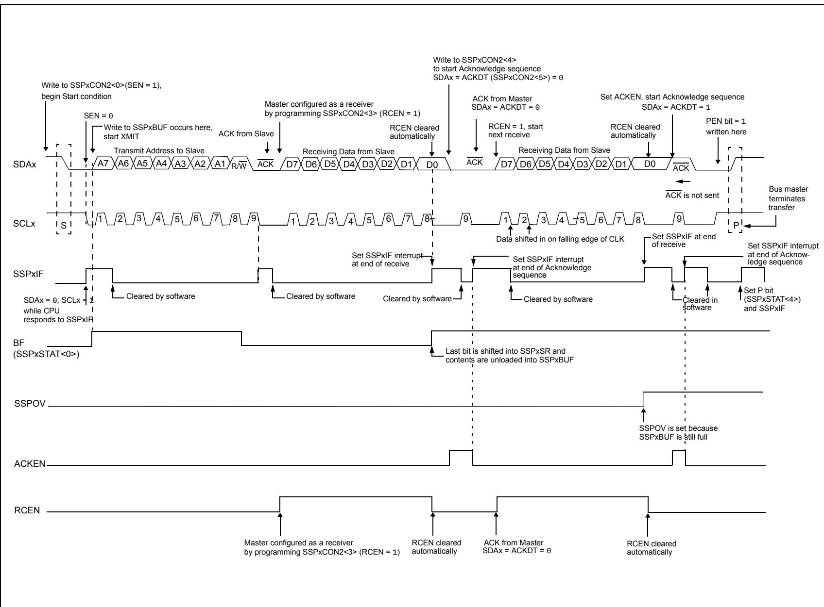
FIGURE 25-29: ^{12}\text{C} MASTER MODE WAVEFORM (RECEPTION, 7-BIT ADDRESS)
