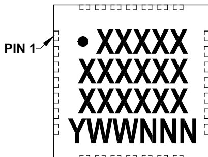
28-Lead UQFN
