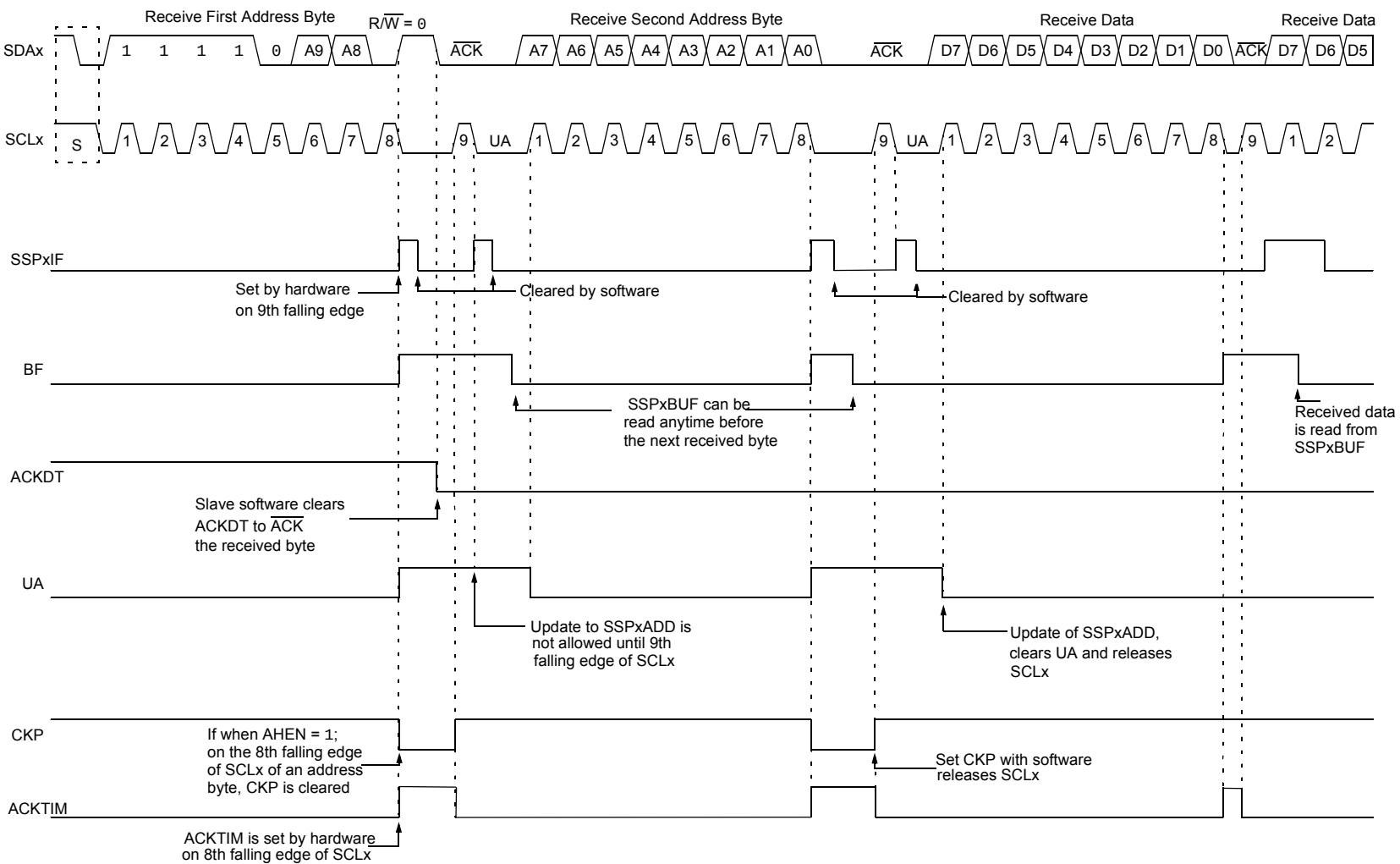
1 2 C SLAVE, 10-BIT ADDRESS, RECEPTION (SEN = 0, AHEN = 1, DHEN = 0)
