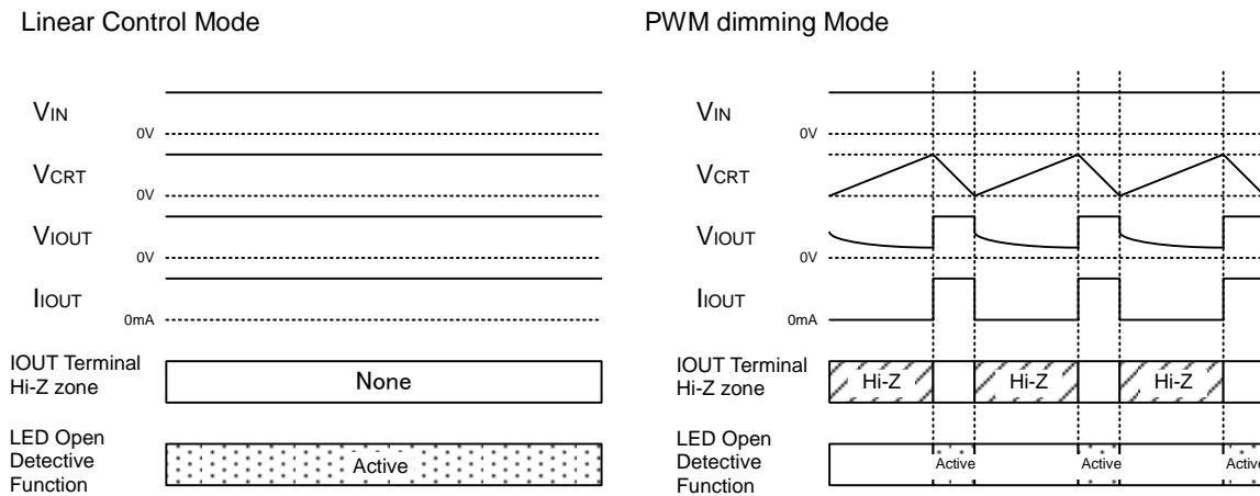
Figure 17. About Active zone of LED Open Detectable Function and IOOUT Terminal Hi-Z zone
