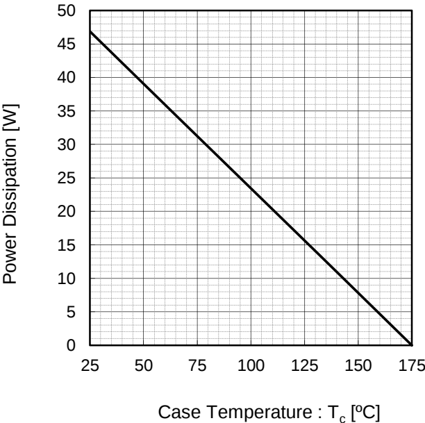
Fig.6 Power Dissipation
