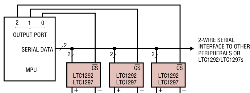
Figure 6. Several LTC1292/LTC1297s Sharing One 2-Wire Serial Interface
