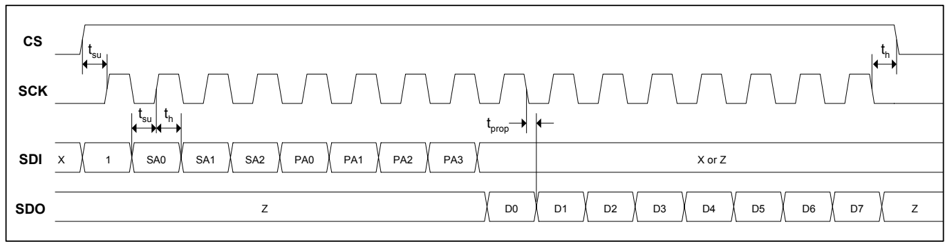
Figure 10: Read Operation
