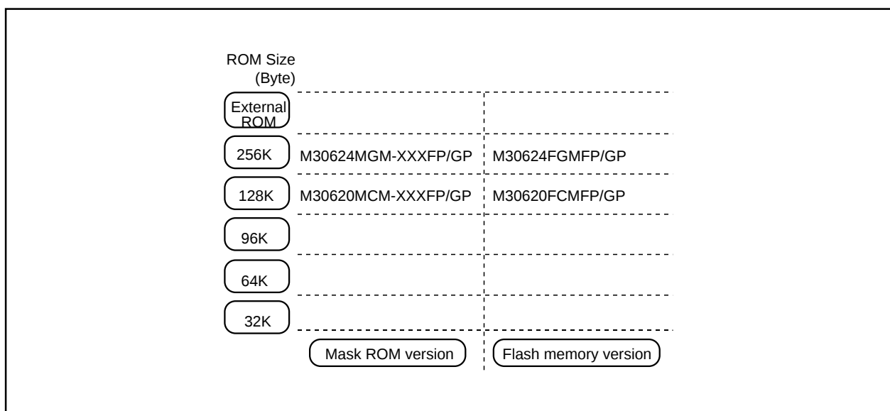
Figure 1.1.4. ROM expansion
