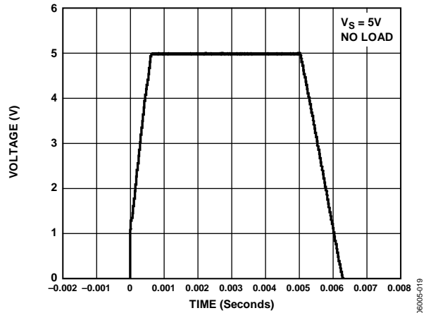
Figure 19. Large Signal Transient Response
