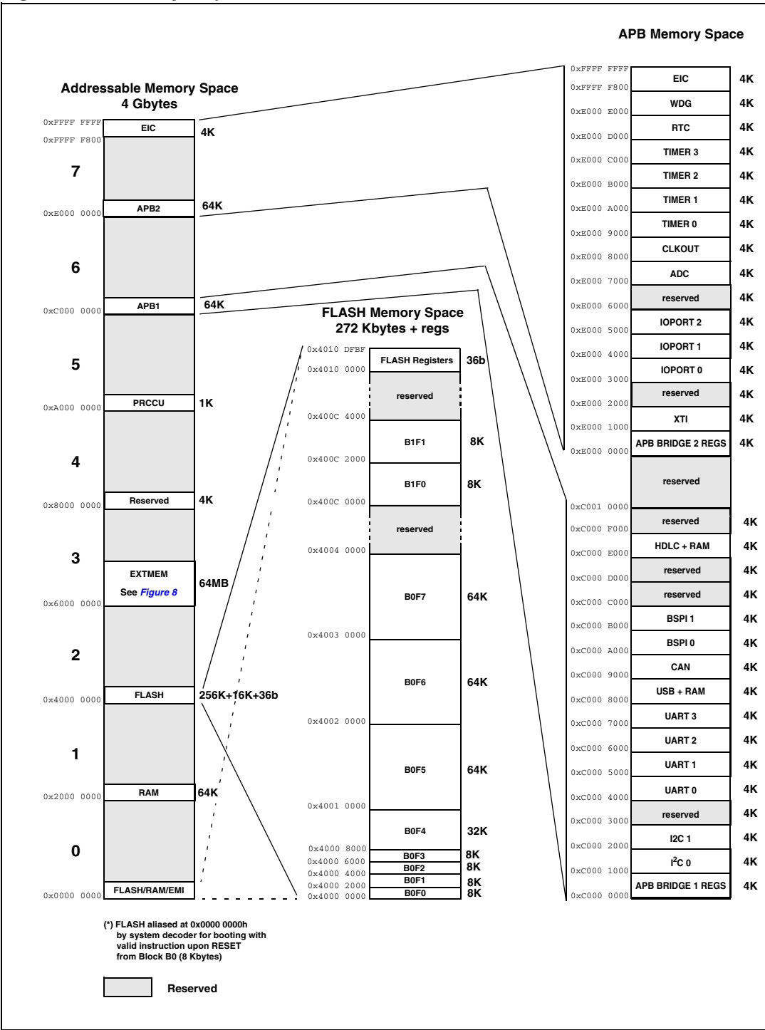
Figure 6. Memory map
