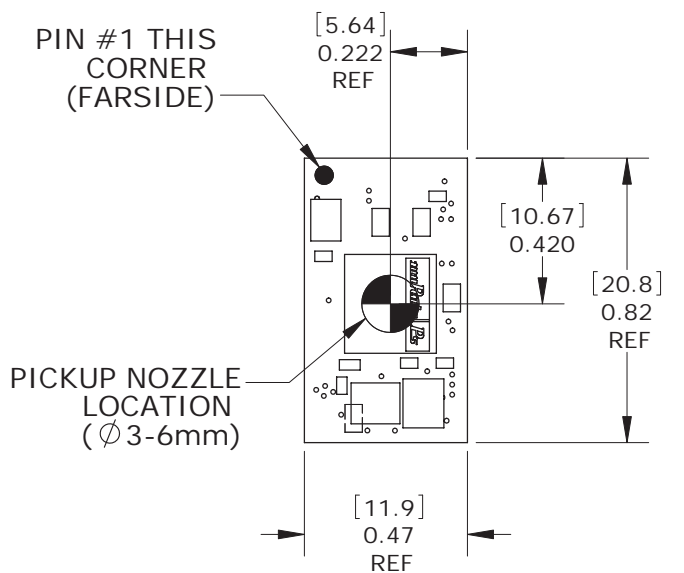
PICK & PLACE PICKUP (P/U)
