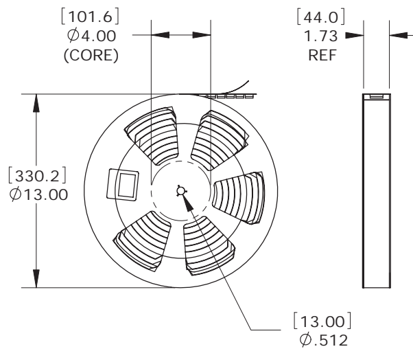
REEL INFORMATION (400 UNITS PER REEL)
