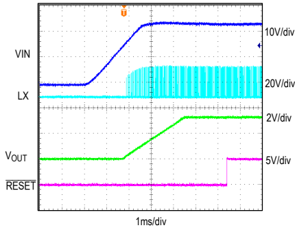
STARTUP THROUGH INPUT SUPPLY VIN = 24V, VOUT = 3.3V, IOUT = 1.7A, MODE = SGND
