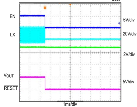
SHUTDOWN THROUGH ENABLE VIN = 24V, VOUT = 5V, IOUT = 0A, MODE = SGND
