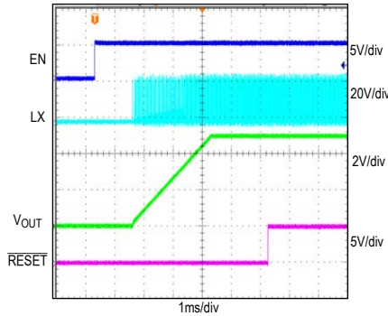
STARTUP THROUGH ENABLE VIN = 24V, VOUT = 5V, IOUT = 0A, MODE = SGND
