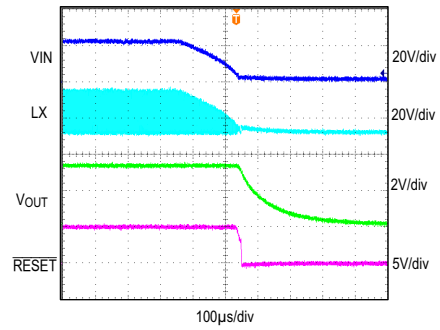
SHUTDOWN THROUGH INPUT SUPPLY VIN = 24V, VOUT = 3.3V, IOUT = 1.7A, MODE = SGND
