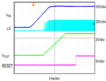
STARTUP THROUGH INPUT SUPPLY VIN = 24V, VOUT = 5V, IOUT = 1.7A, MODE = SGND
