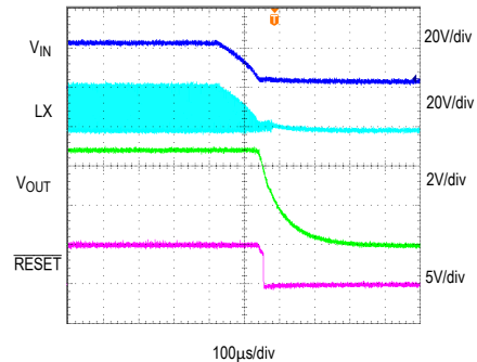
SHUTDOWN THROUGH INPUT SUPPLY VIN = 24V, VOUT = 5V, IOUT = 1.7A, MODE = SGND
