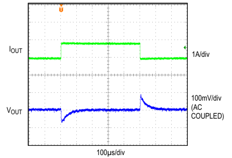
LOAD CURRENT TRANSIENT RESPONSE V_{IN} = 24V, V_{OUT} = 5V, I_{OUT} = 0.05A - 0.85A, MODE = SGND
