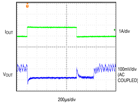
LOAD CURRENT TRANSIENT RESPONSE V_{IN} = 24V, V_{OUT} = 5V, I_{OUT} = 0.05A - 0.85A, MODE = OPEN
