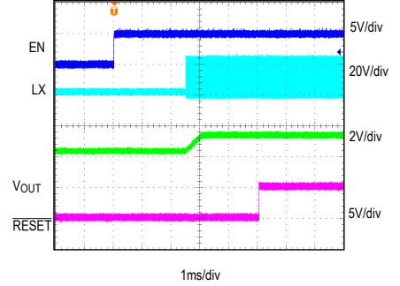
STARTUP WITH 2.5V PREBIAS V_{IN} = 24V, V_{OUT} = 3.3V, I_{OUT} = 0A, MODE = SGND
