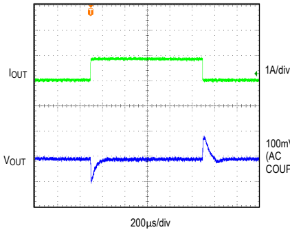
LOAD CURRENT TRANSIENT RESPONSE V_{IN} = 24V, V_{OUT} = 3.3V, I_{OUT} = 0.05A - 0.85A, MODE = VCC
