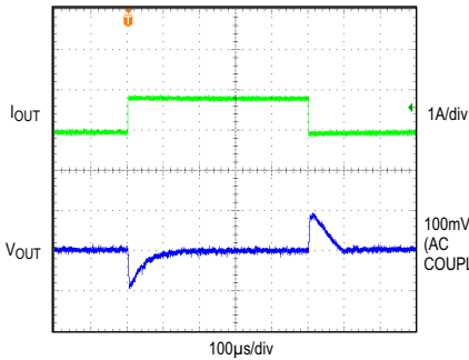
LOAD CURRENT TRANSIENT RESPONSE V_{IN} = 24V, V_{OUT} = 5V, I_{OUT} = 0.05A - 0.85A, MODE = VCC
