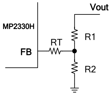
Figure 4: Feedback Network
