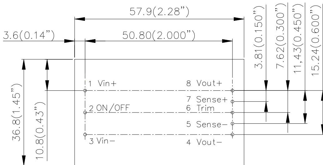
TOP VIEW
