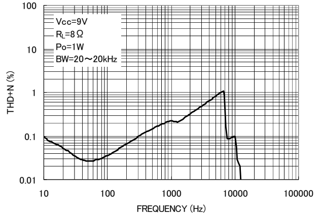
Fig. 2 THD+N - Frequency
